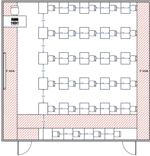
960 Sq Ft Layout: 3 feet distance (29 students)
