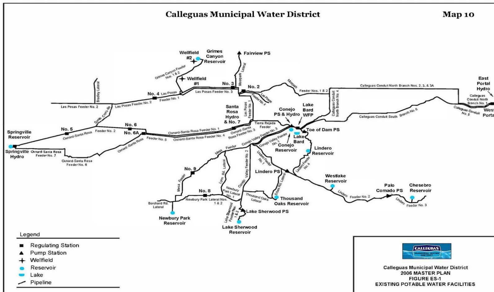
Figure 3-11a Calleguas Municipal Water District Major Infrastructure WCVC IRWM Region
