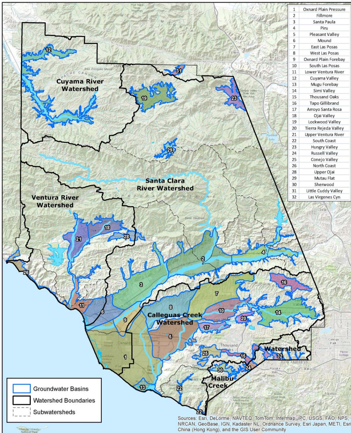
Figure 3-8 Groundwater Basins WVCV IRWM Region
