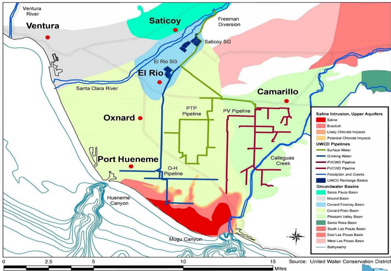
Figure 3-16 Seawater Intrusion Levels WVCV IRWM Region
